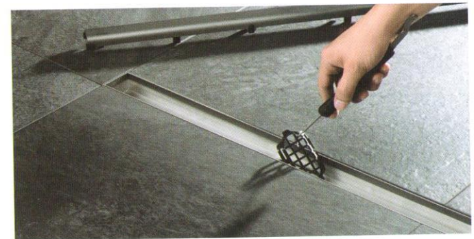
Grates and dirt traps are easy to remove using the Viega Advantix multi-tool.
